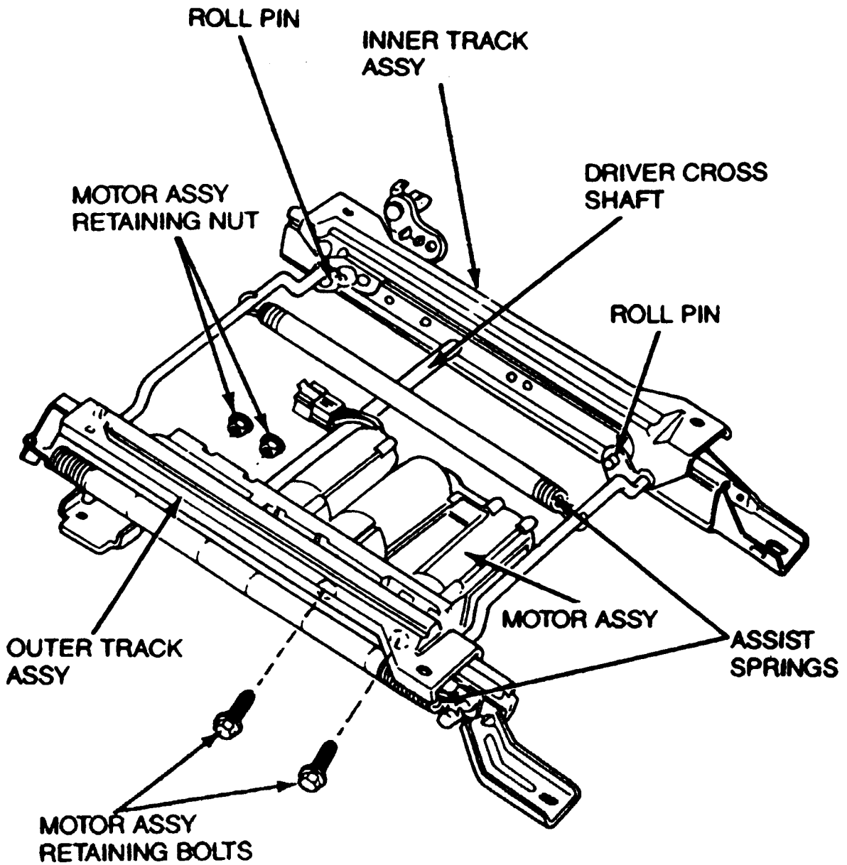
PASSENGER SEAT SHOWN DRIVER SEAT TYPICAL
