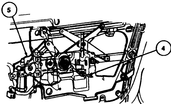
ELECTRIC REGULATOR INSTALLATION
