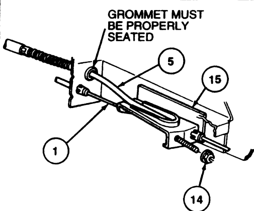
VIEW V
