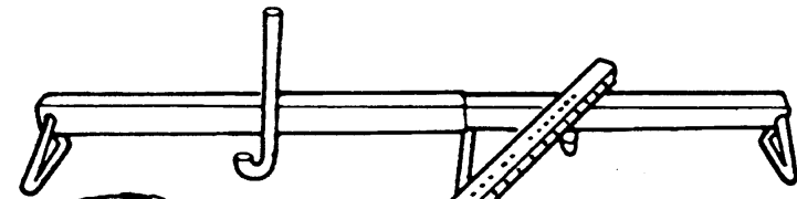
THREE BAR ENGINE SUPPORT D87L-6000-A
