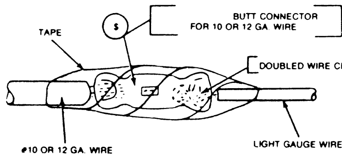
TYPICAL REPAIR ATTACHING THREE LIGHT GAUGE FUSE LINKS TO A SINGLE HEAVY GAUGE FEED WIRE
