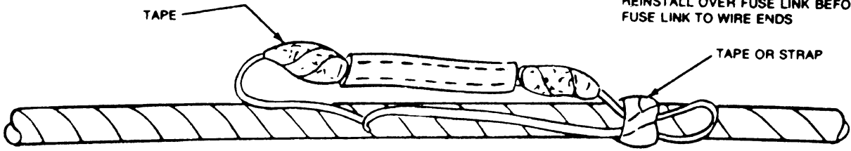
TYPICAL REPAIR USING THE SPECIAL #17 GA. (9.00' LONG-YELLOW) FUSE LINK REQUIRED FOR THE AIR/COND. CIRCUITS
