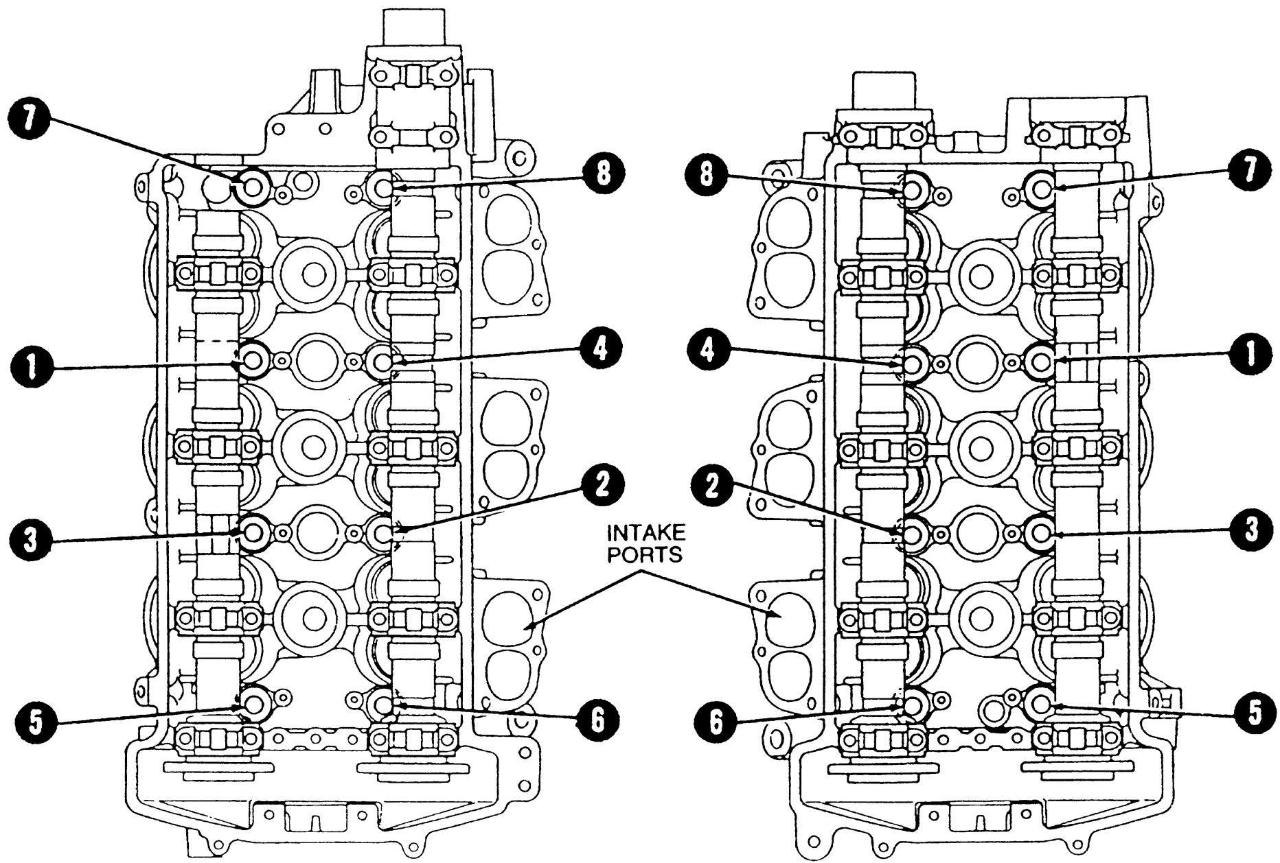
TIGHTEN CYLINDER HEAD BOLTS IN THE ORDER SHOWN
