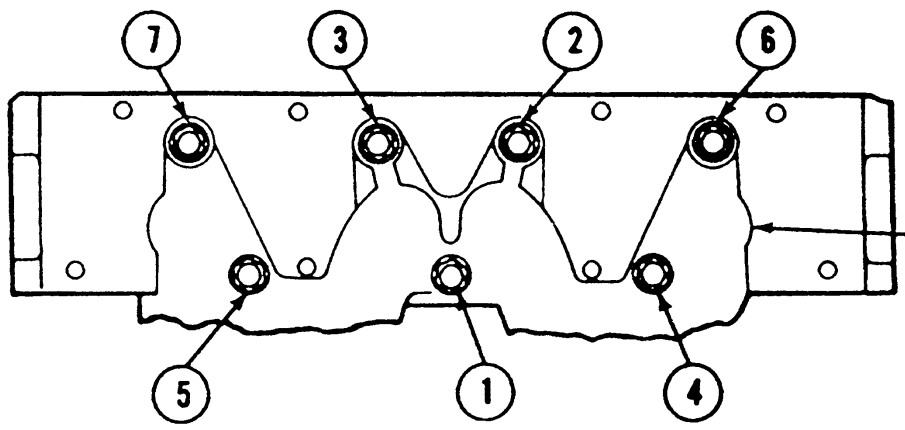
BOLT TIGHTENING SEQUENCE (TWO STAGES)
