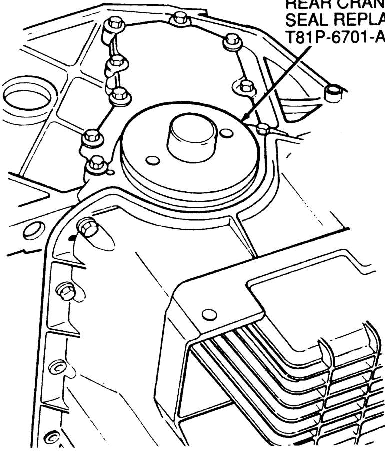
REAR SEAL REPLACER SCREW SET T89P-6701-C
