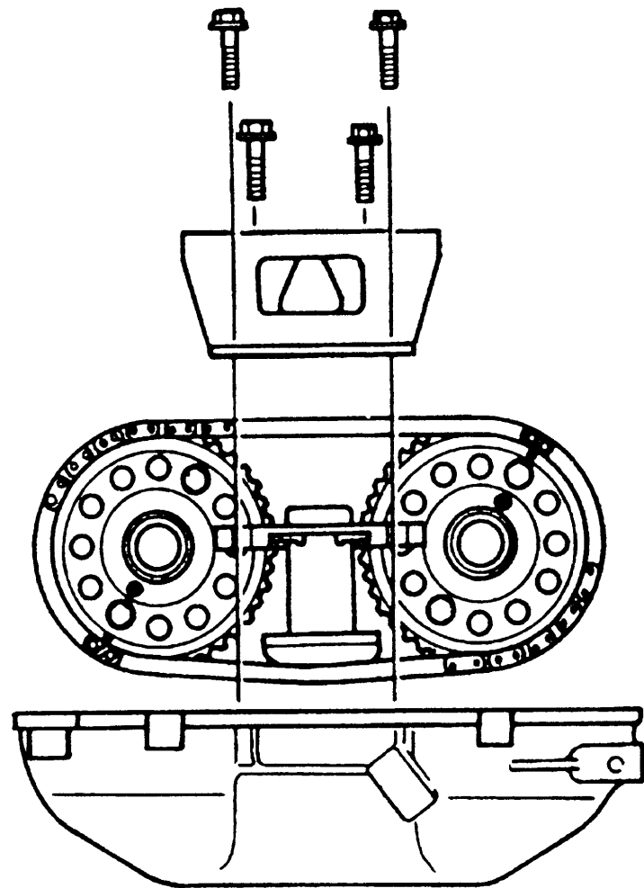
RH TIMING CHAIN TENSIONER 6K261
